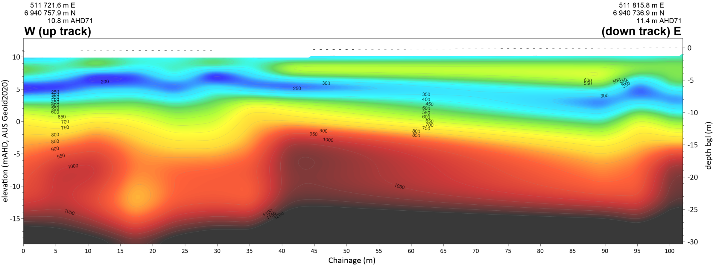
Seismic Line MASW AU-GP 140
